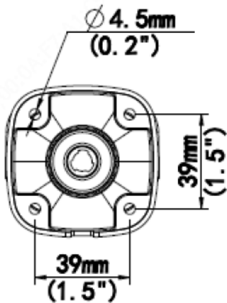
XLGUP06-B Pole Mount
